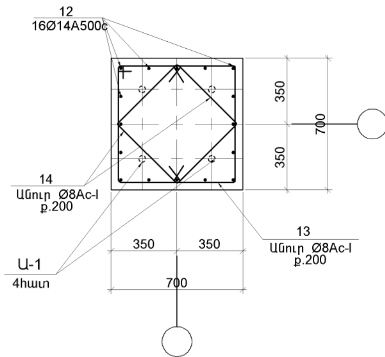
1 - 1 (M1:20)
