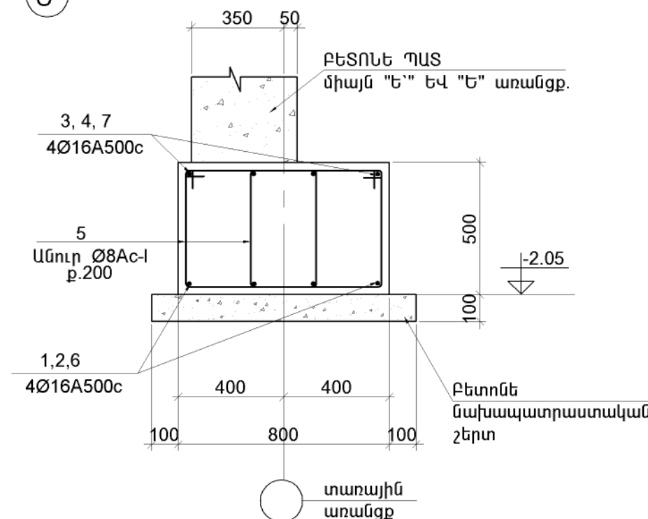
1 - 1 (M1:20)
